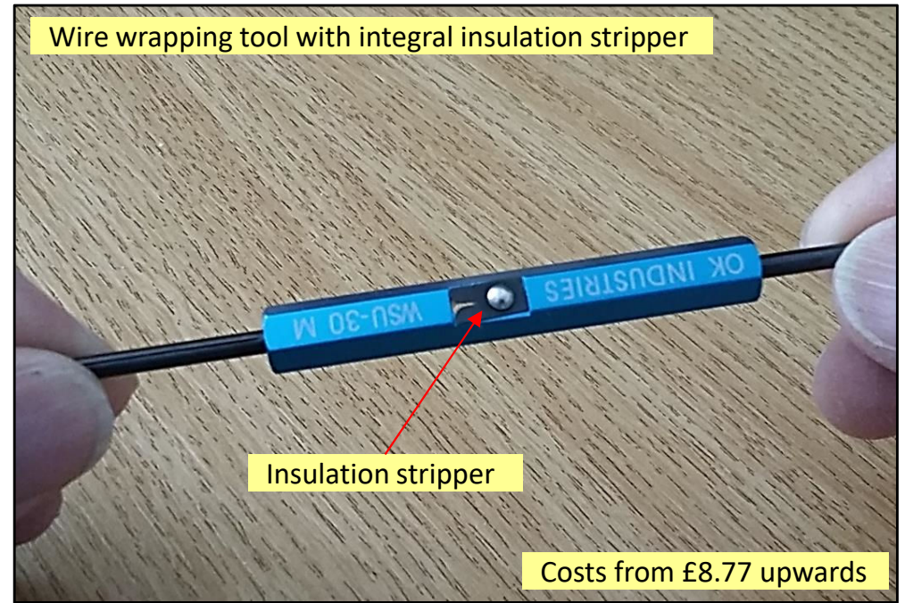
Cut wire to length and feed end through hole in stripper
